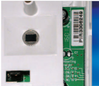
Mounting Height Adjustment
